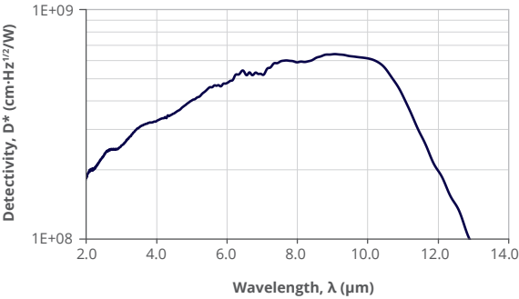
PC-4TE-10.6-1x1-TO8/TO66-wZnSeAR-70
